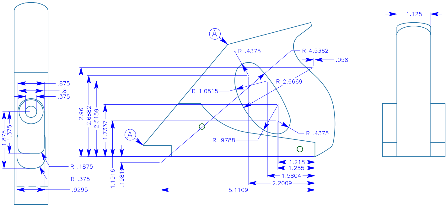
Adjuster Mortise View from A-A
